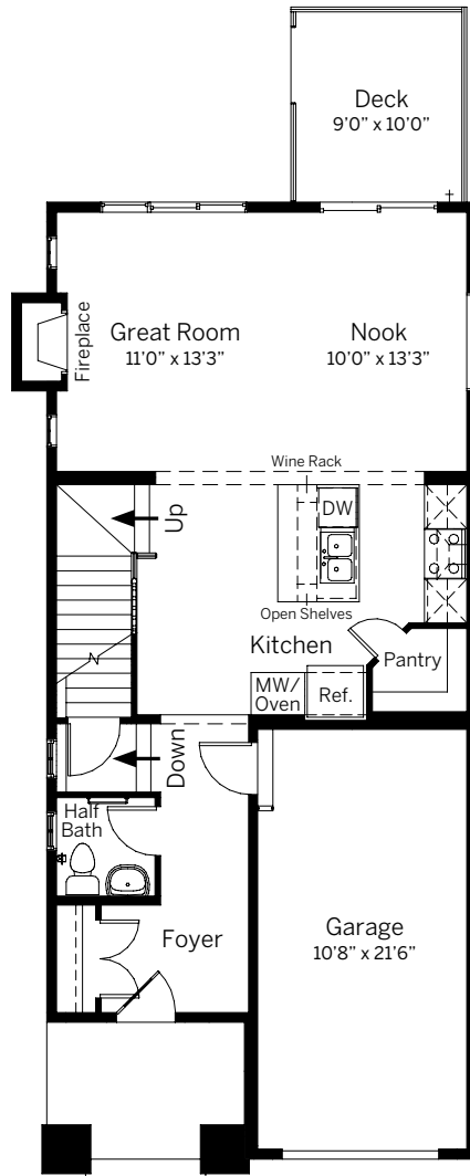
MAIN FLOOR 756 sq. ft.
