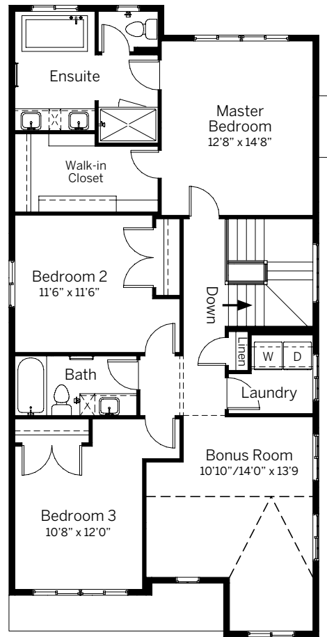
SECOND FLOOR 1277 sq. ft.
