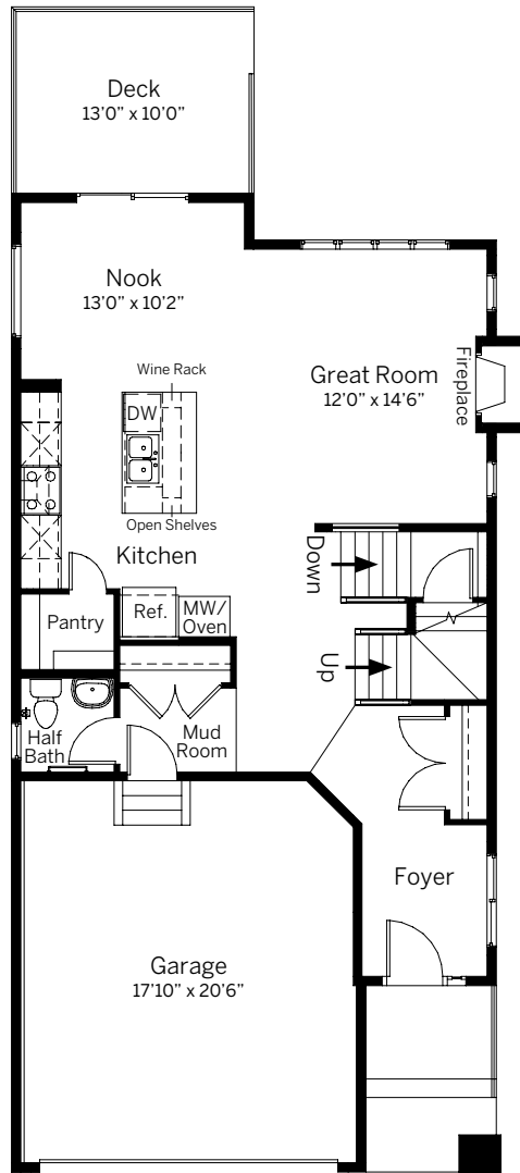
MAIN FLOOR 874 sq. ft.
