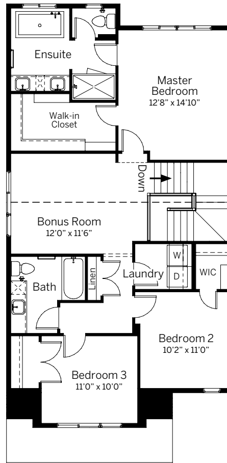
SECOND FLOOR 1173 sq. ft.
