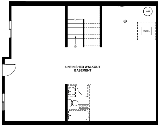
Unfinished Basement
