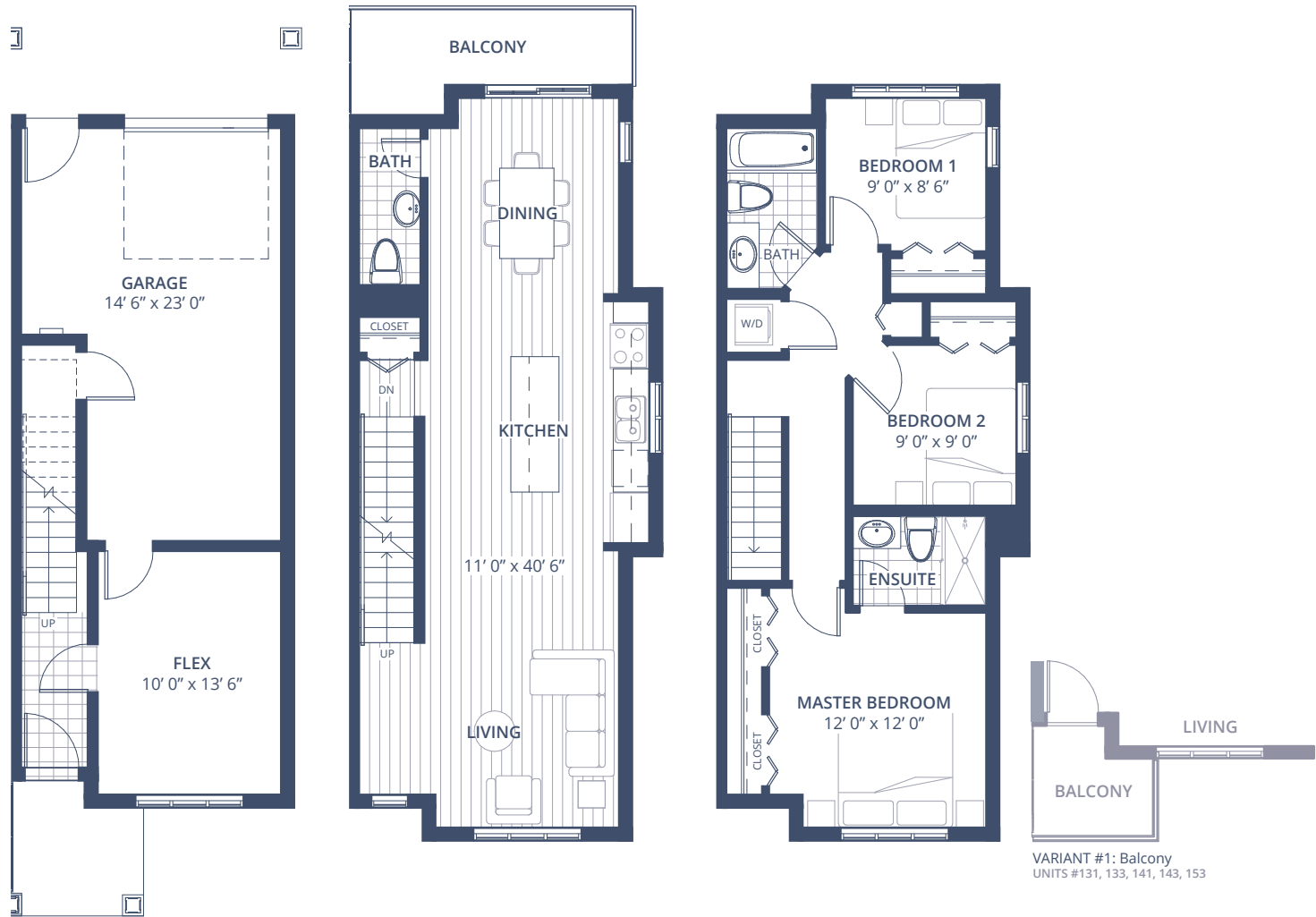
LOWER FLOOR 225 sq ft
