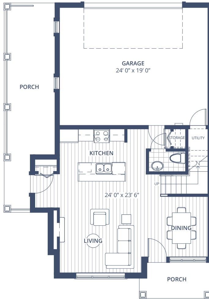
LOWER FLOOR 624 sq ft
