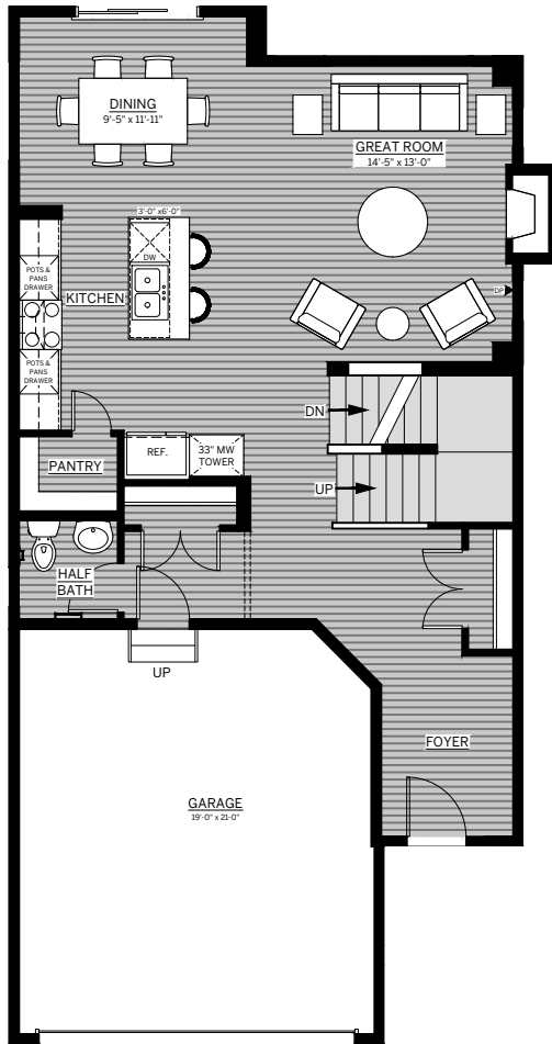
MAIN FLOOR 875 sq. ft.
