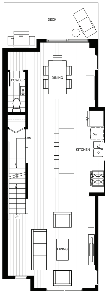
MAIN FLOOR
