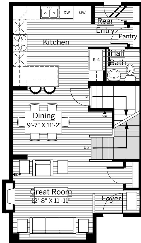
MAIN FLOOR 692 sq. ft.
