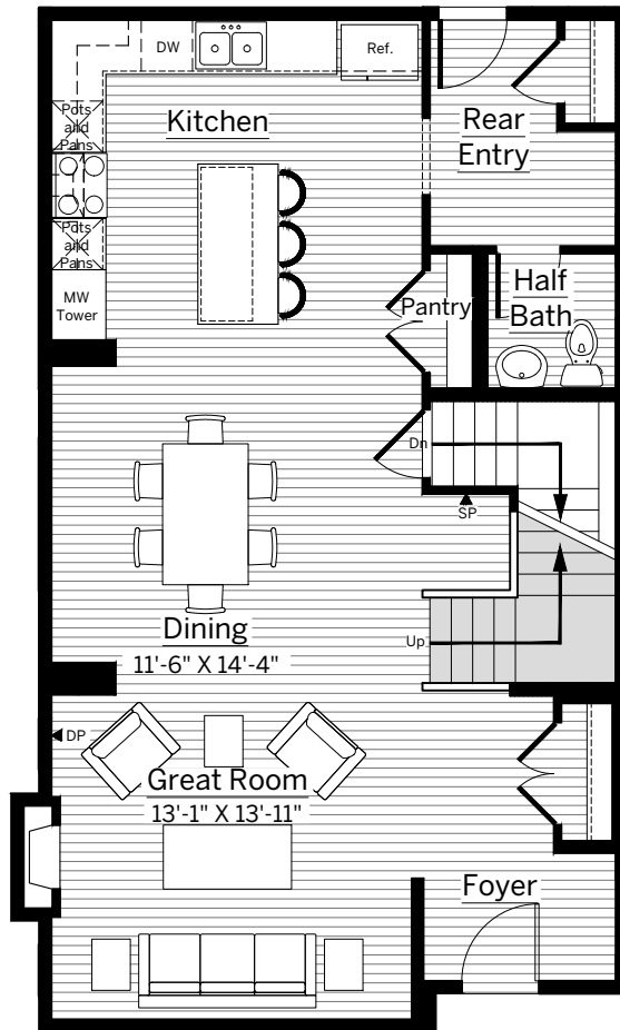
MAIN FLOOR 908 sq. ft.
