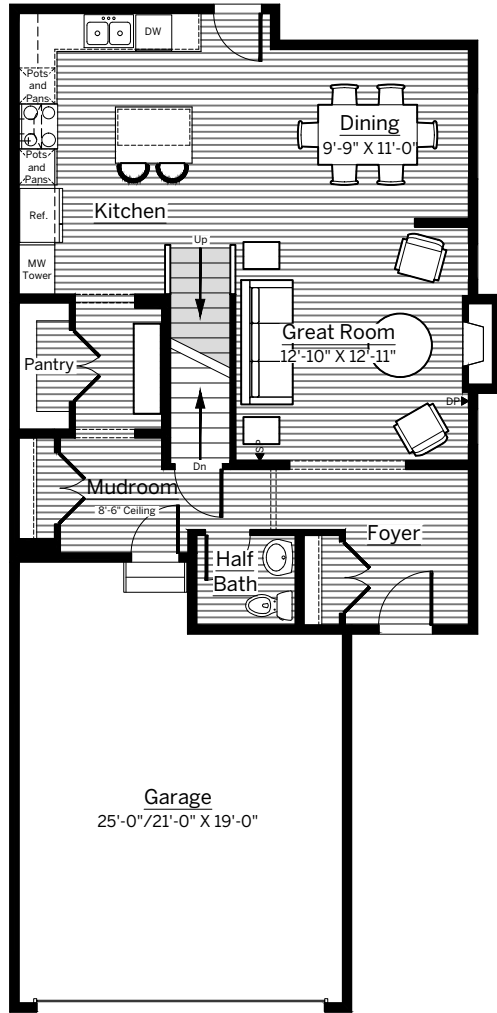
MAIN FLOOR 849 sq. ft.
