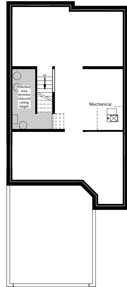
UNFINISHED BASEMENT 936 sq. ft.
