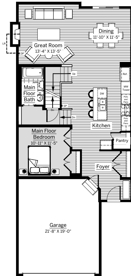
MAIN FLOOR 1053 sq. ft.
